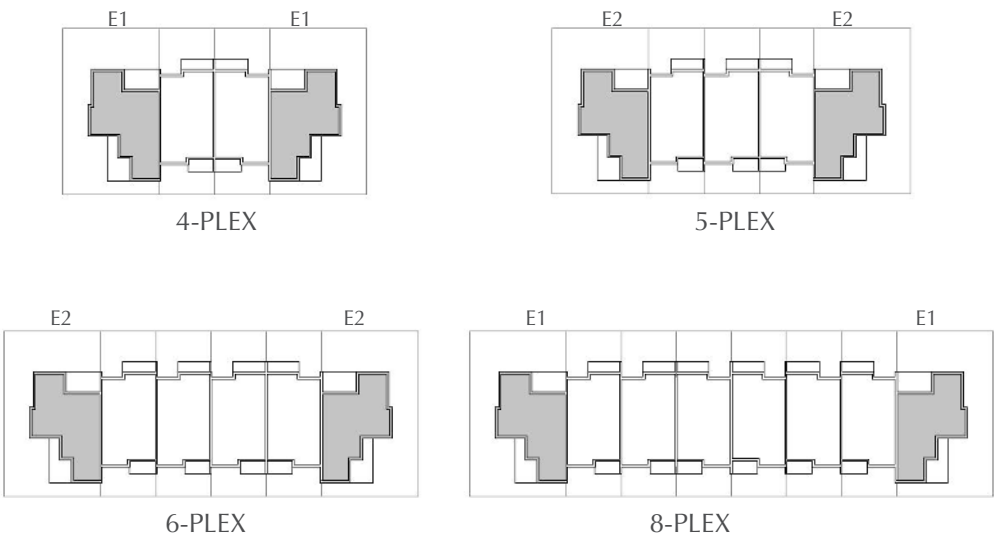
KEY PLAN
