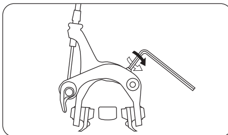
Setting up the distance between the brakes and the rim
