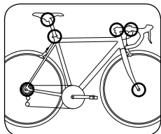
Possible positions of quick release skewers, through axles and screw connections
