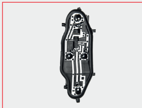
ASSEMBLY WITH WELDING (WITH ELECTRICAL TEST)
