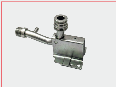
ASSEMBLY WITH BRAISING (WITH LEAK TEST)
