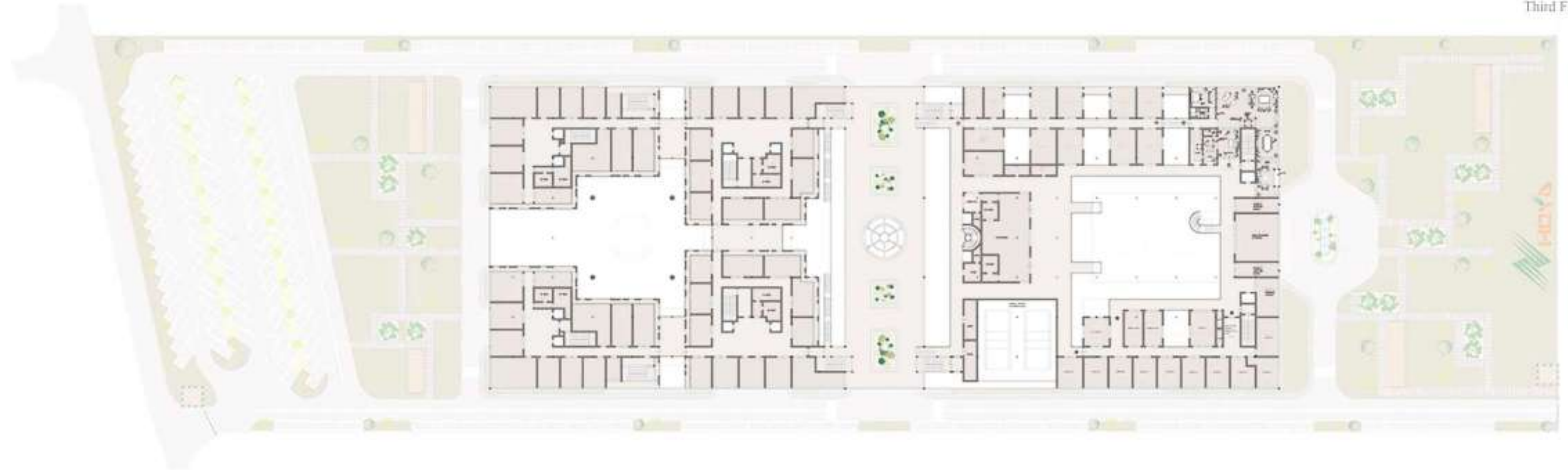
General Layout Plan Roof
