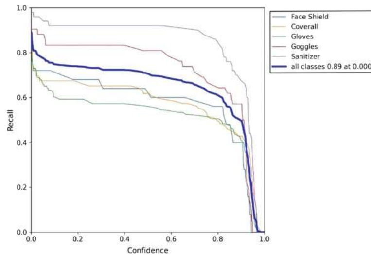
Fig. 7.12 Recall versus confidence
