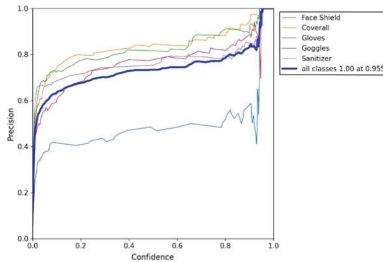
Fig. 7.10 Precision versus confidence
