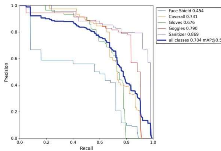
Fig. 7.11 Precision versus recall
