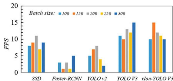
Fig. 7.2 FPS versus batch size for five popular detection algorithms (Li et al., 2020)
