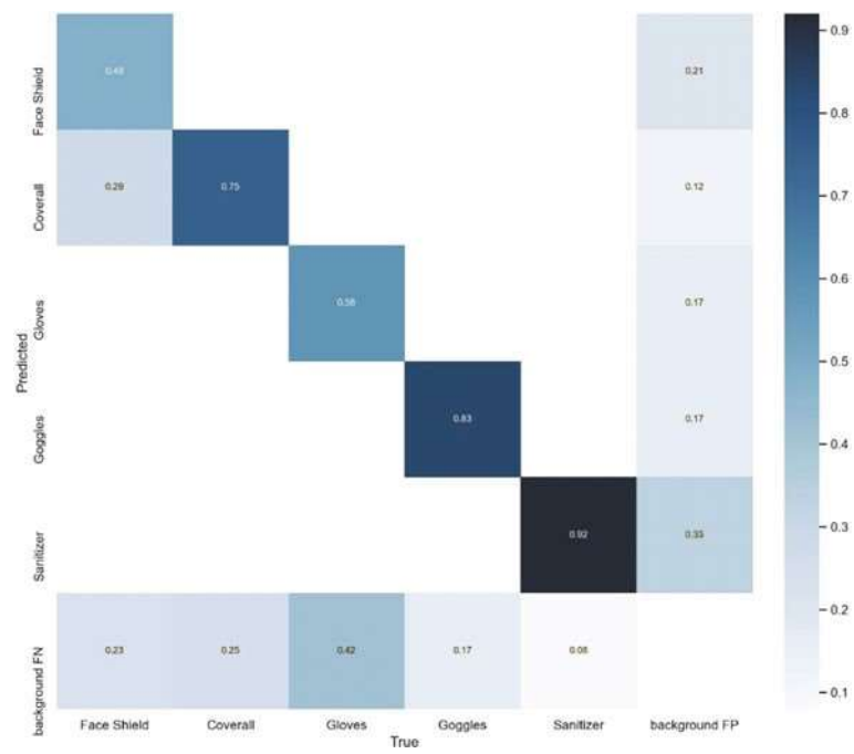
Fig. 7.8 Confusion matrix across PPE object classes
