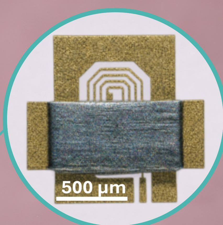
Micro-magnet on an RF planar inductor
