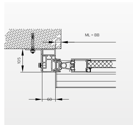
Wandmontage
