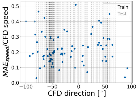
(c) MAE_{speed} scaled with CFD wind speed versus CFD wind direction.
