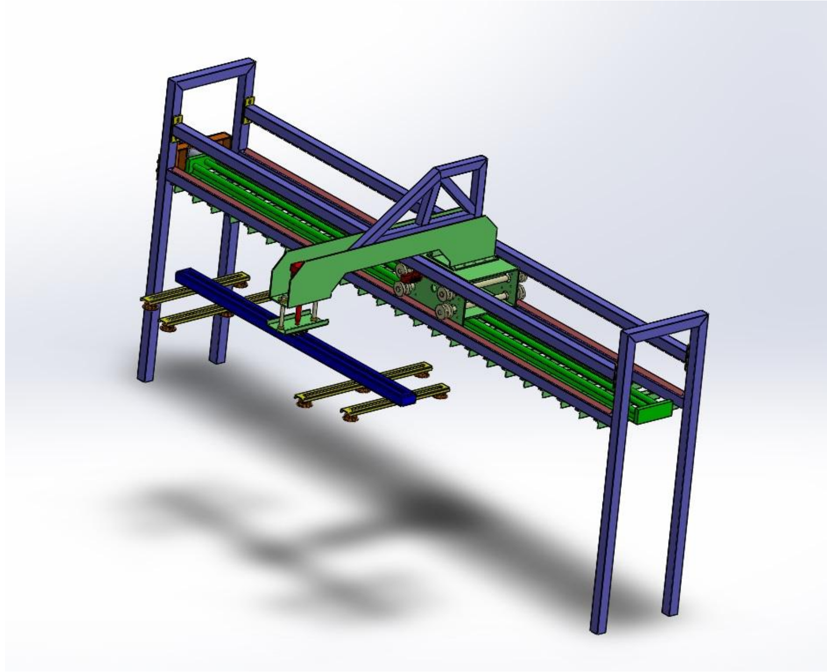
VACUUM MANIPULATOR
