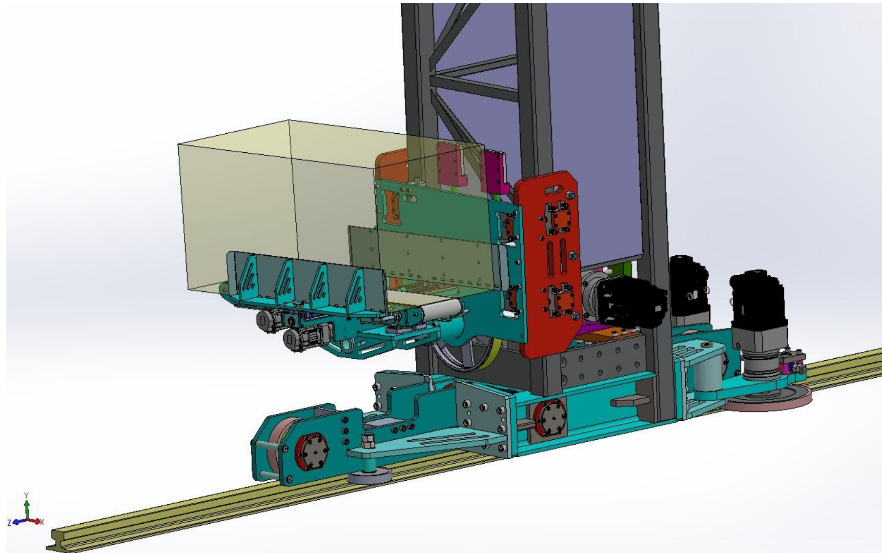
LOADING ROBOT
