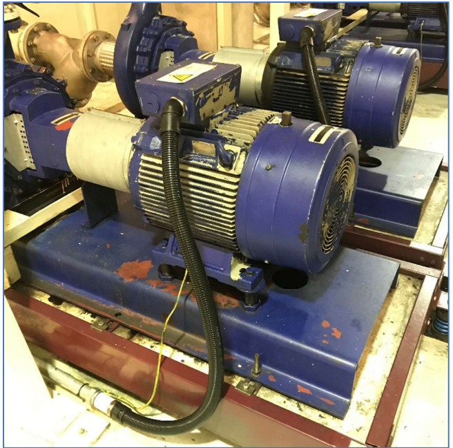
Change of 35mm 2 wiring, wire protection and Siemens switch (before vs. after)
