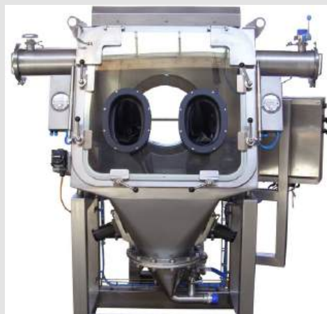
DRUM DISCHARGING
