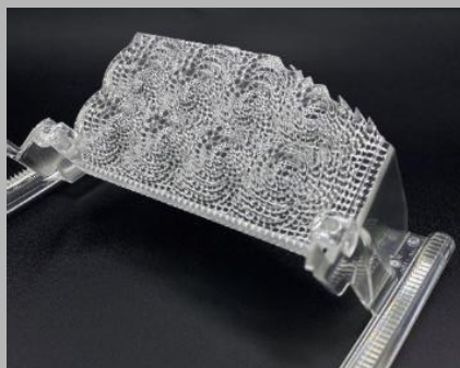
Lightguide with milled fresnel & pillow optics
