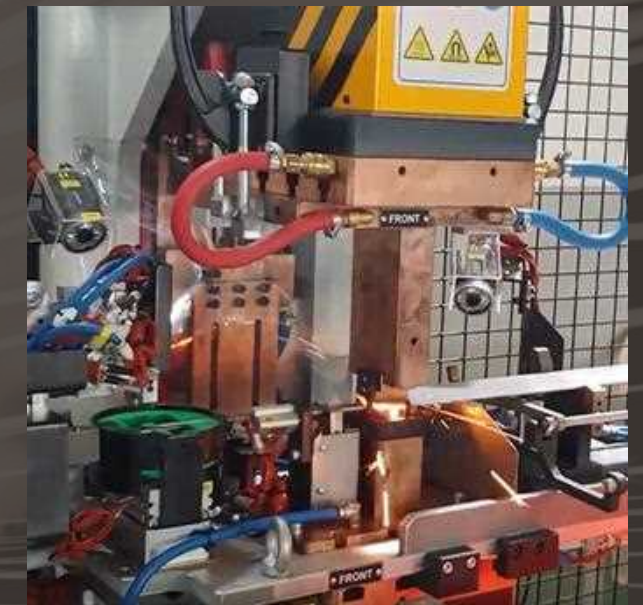
Fuel Tank Belt Welding Machine
