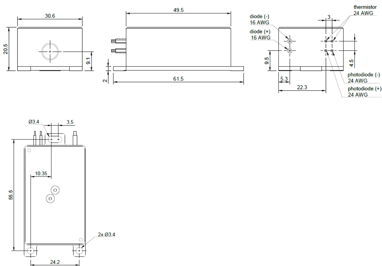
Figure 1. Laser head.
