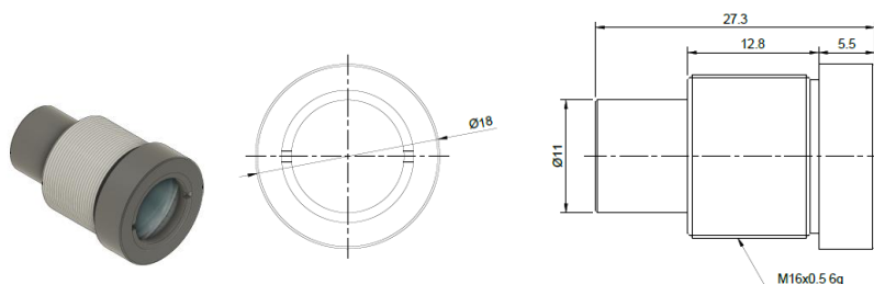
Figure 3. Collimator as separate component (not mounted).
