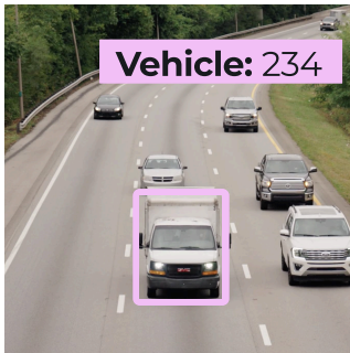
Traffic Analytics
