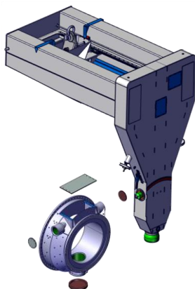
Spacecraft Horizontal Hoisting Device with spacecraft Integration Spacer
