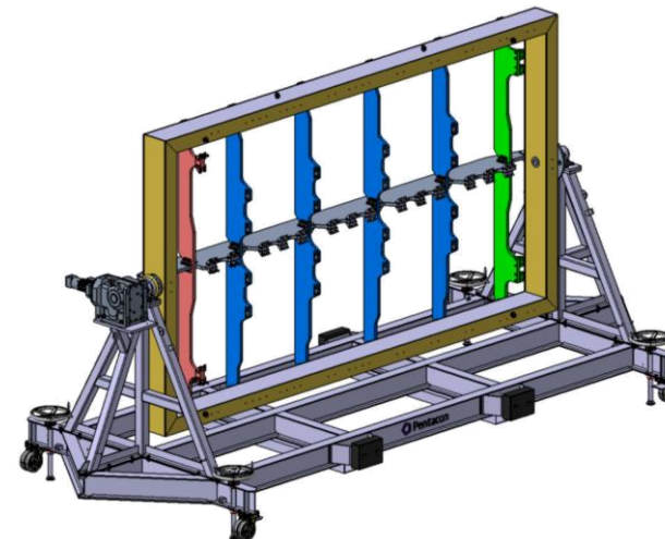
Satellite Service module Simulator (PFM&FM)
