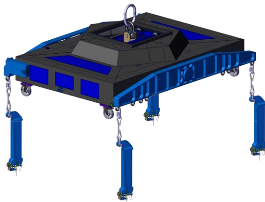
Spacecraft Horizontal Hoisting Device with spacecraft Integration Spacer
