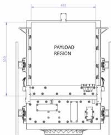
FRONT VIEW: PAYLOAD DIMENSION
