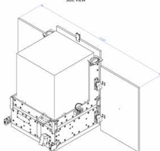
VIEW: DEPLOYED SOLAR PANEL
