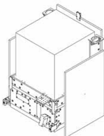
VIEW: STOWED SOLAR PANEL
