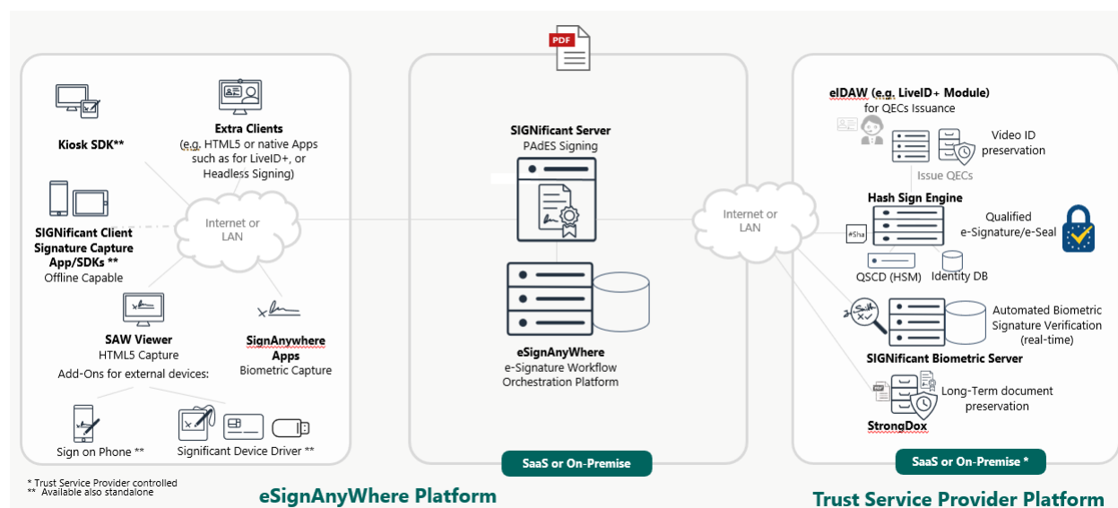
eSignAnyWhere platform architecture
