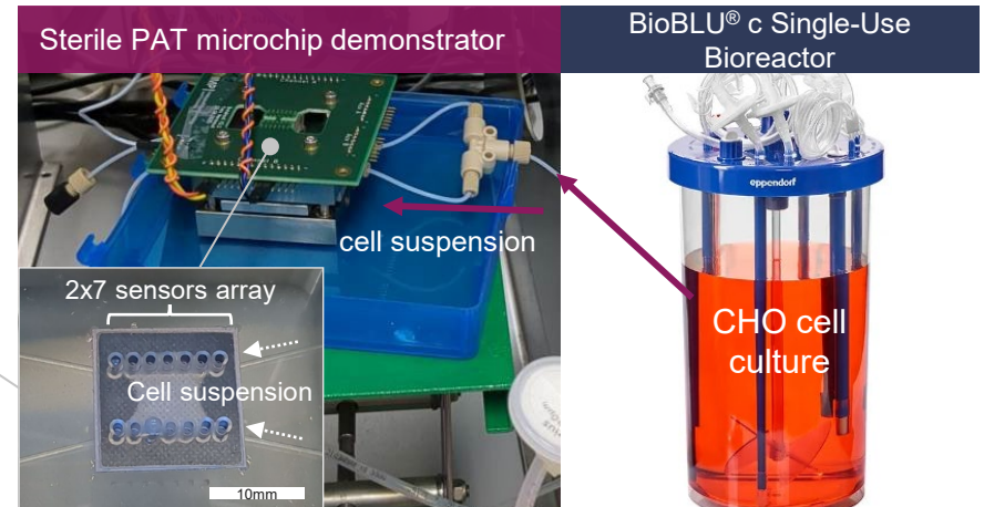
Proof of concept in 300ml bioreactor
