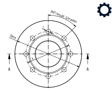
Insulating flange connections for customised solutions
