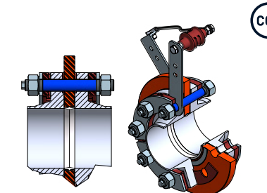
Insulating flanges for aggressive and critical media
