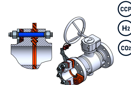
Insulating flanges for valves and vessels
