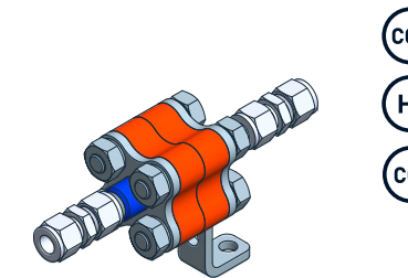
ISO-KonneX insulating flanges for screw-type connection systems (clamping, cutting ring)
