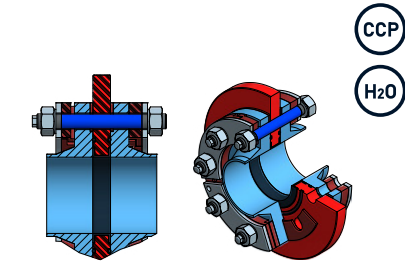
Insulating flanges for drinking water
