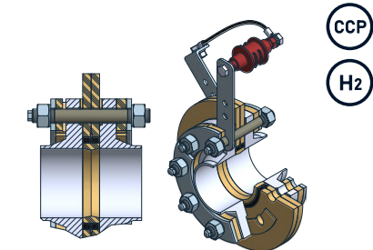
Insulating flanges for high temperatures up to +260 °C (HTB approval)
