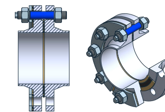
Electrical isolation for stainless steel separation (galvanic isolation)
