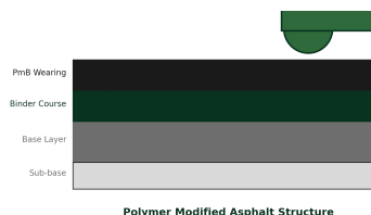
Polymer Modified Asphalt Structure
