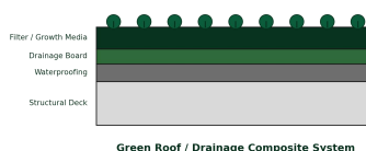
Green Roof / Drainage Composite System
