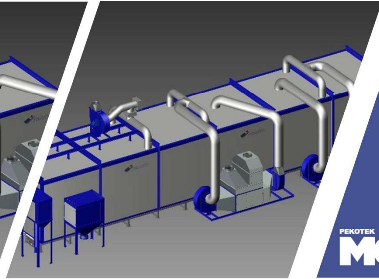
3. Added painting + drying unit
