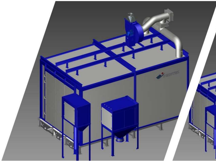
1. Combined blasting + painting unit
