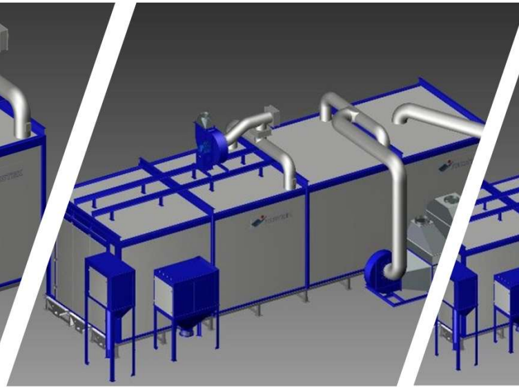
2. Added painting unit
