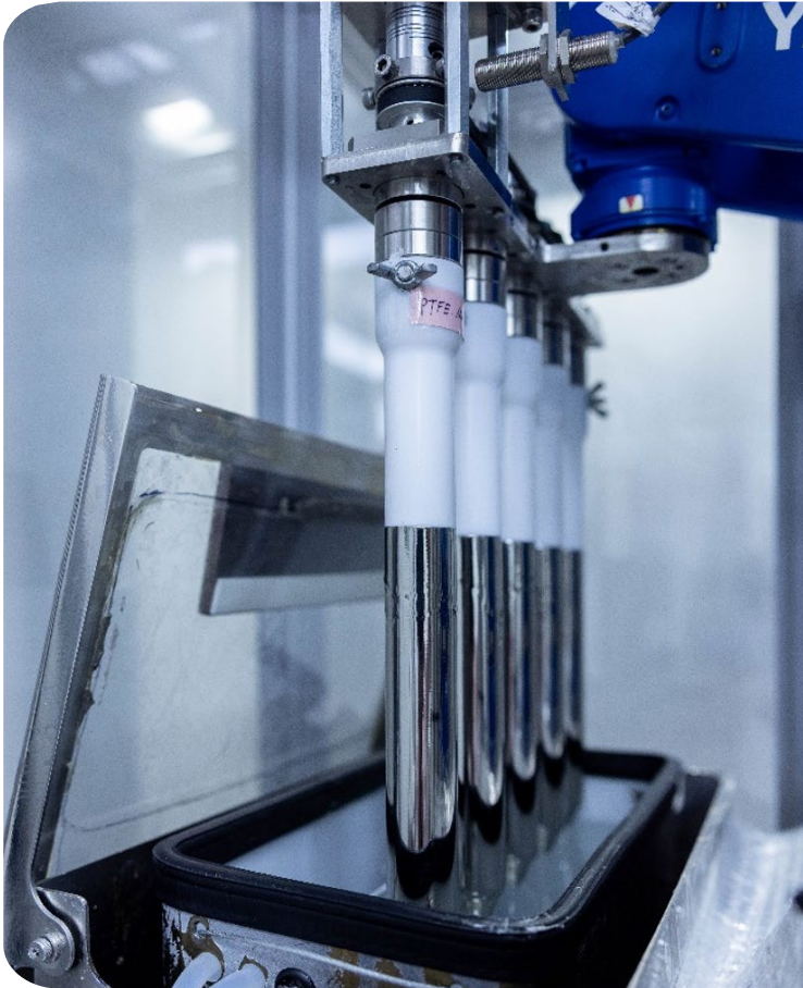
Eudaemon Technologies Pilot production machine for skin-like condoms made from tough hydrogels (Sydney, Australia)
