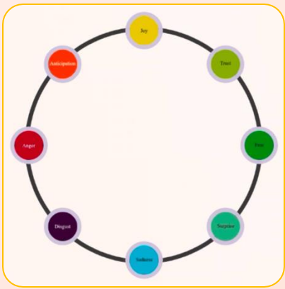
Emotion Score
