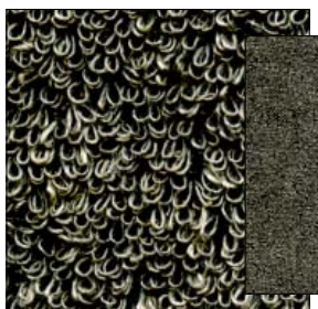
CL817, 590 ± 55 g/m 2 , loops 100 % linen base 100 % cotton, width 235 ± 5 cm
