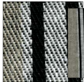
LL165J, 330 ± 35 g/m 2 , 100 % linen, width 150 ± 5 cm
