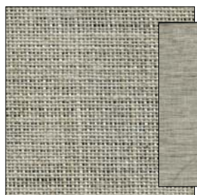
LL27N, 270 ± 25 g/m 2 , 100 % linen, width 150 ± 5 cm
