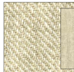
LL026T, 340 ± 35 g/m 2 , 100 % linen, width 75 ± 5 cm
