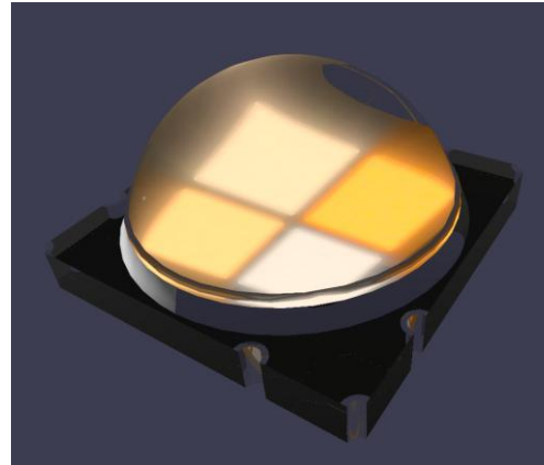
LightTools
