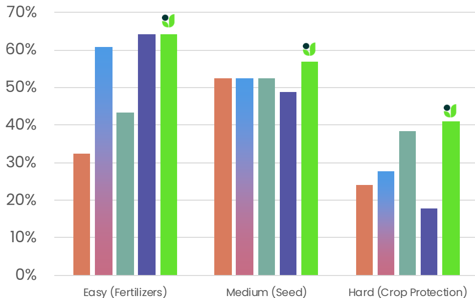
Accuracy over agronomy Q&A dataset
