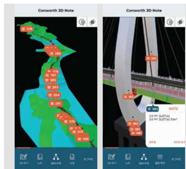
3D Note (Bridge Construction Site)
