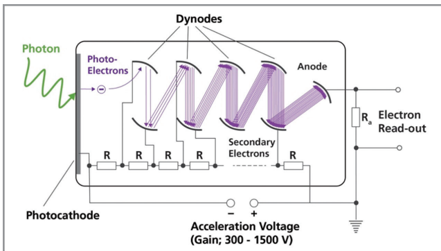
Figure 2: Schematic of a Typical Photomultiplier
