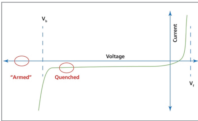
Figure 5: Current vs. voltage diagram of an APD, showing “armed” and “quenched” states
