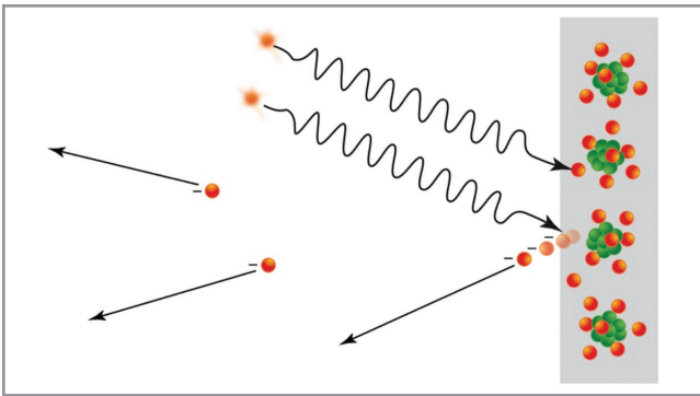
Figure 1: The photoelectric effect in a solid
