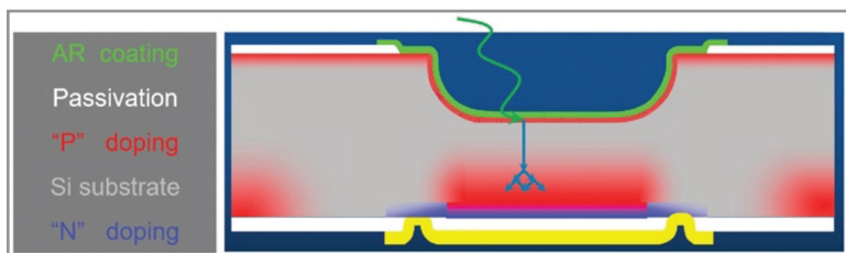
Figure 3: A typical APD structure
