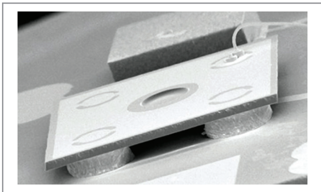
Figure 4: The SLiK Avalanche Photodiode, optimized for single photon detection
