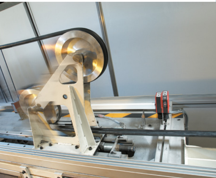
BENDING TEST
