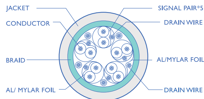
HDMI Coaxial Structure
