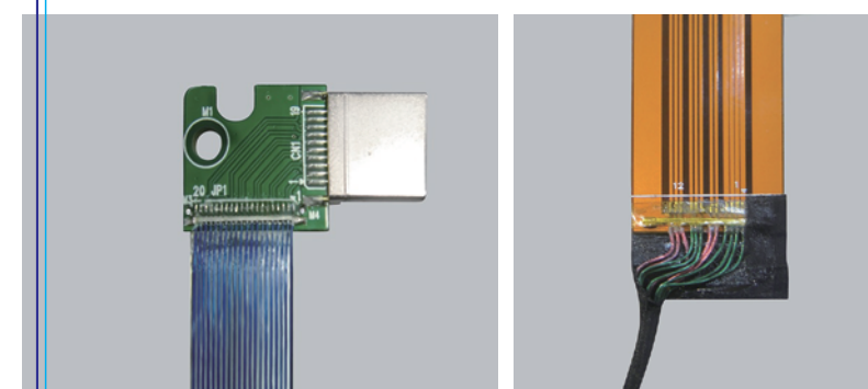
Coax cable connecting to PCB with SMD method.
