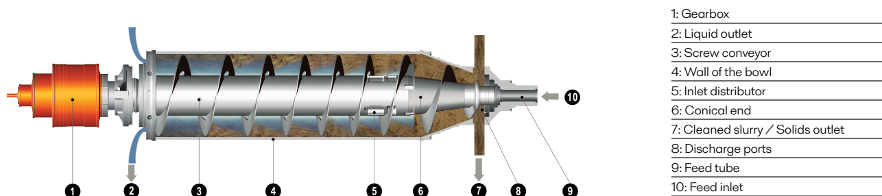
Cross section of the interior of the decanter - the rotating assembly
