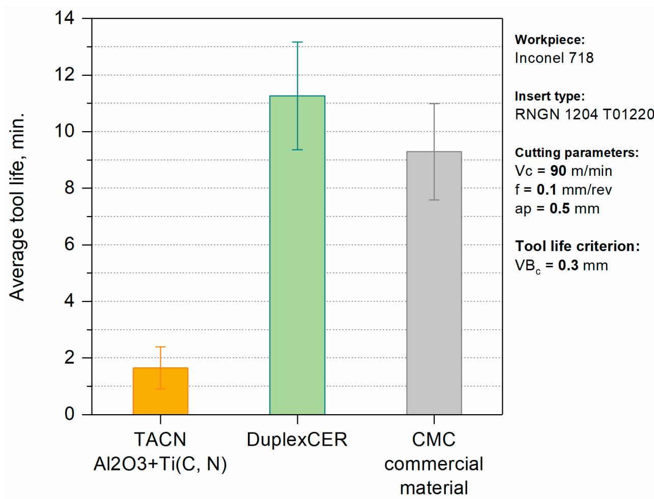
Tool life
