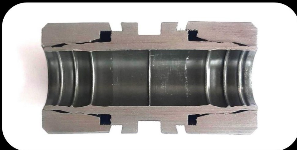
Fitting : Cross view of the body and 2 press rings
