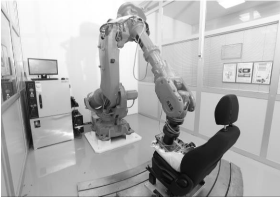
Static Test
