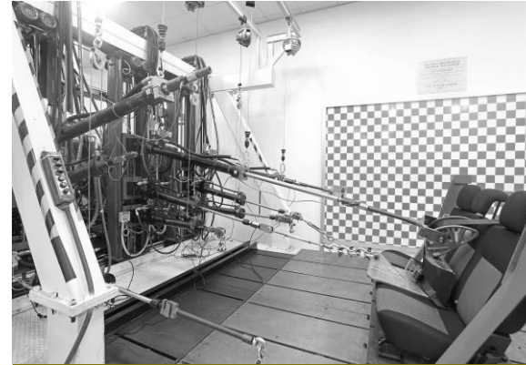
Pulling Strength Test
