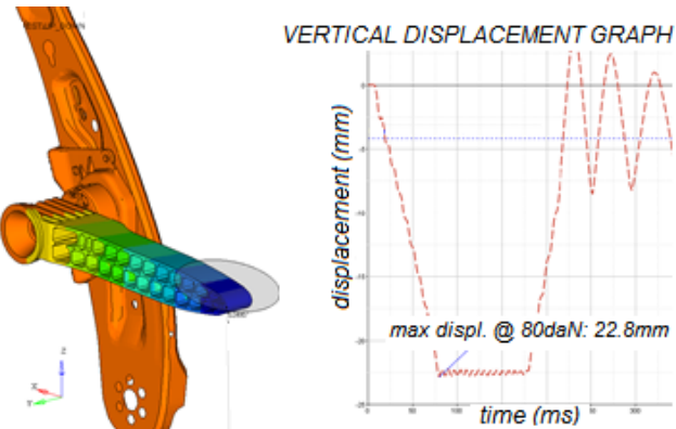
Armrest Static Loading
