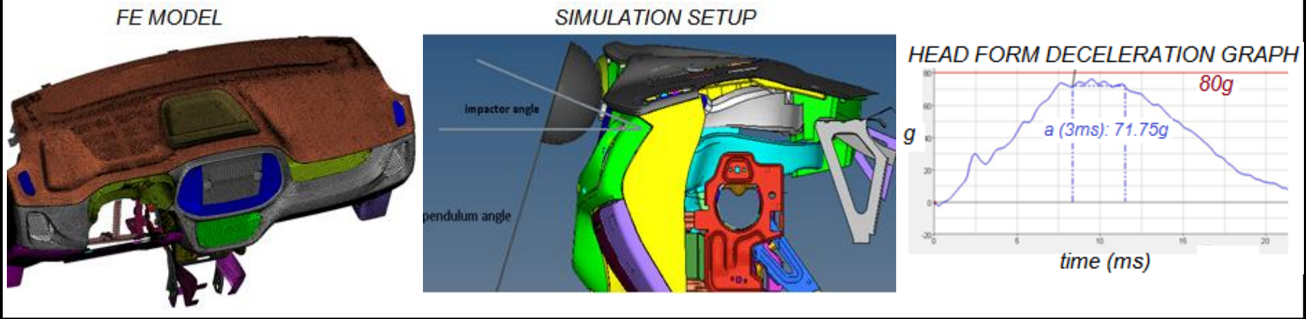
Sunvisor frame topology optimization
