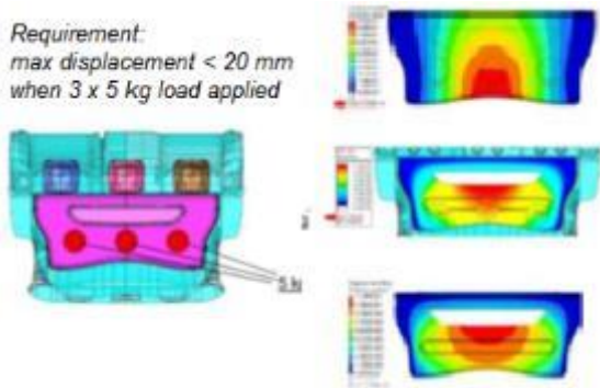
Parcel Tray Static Loading
