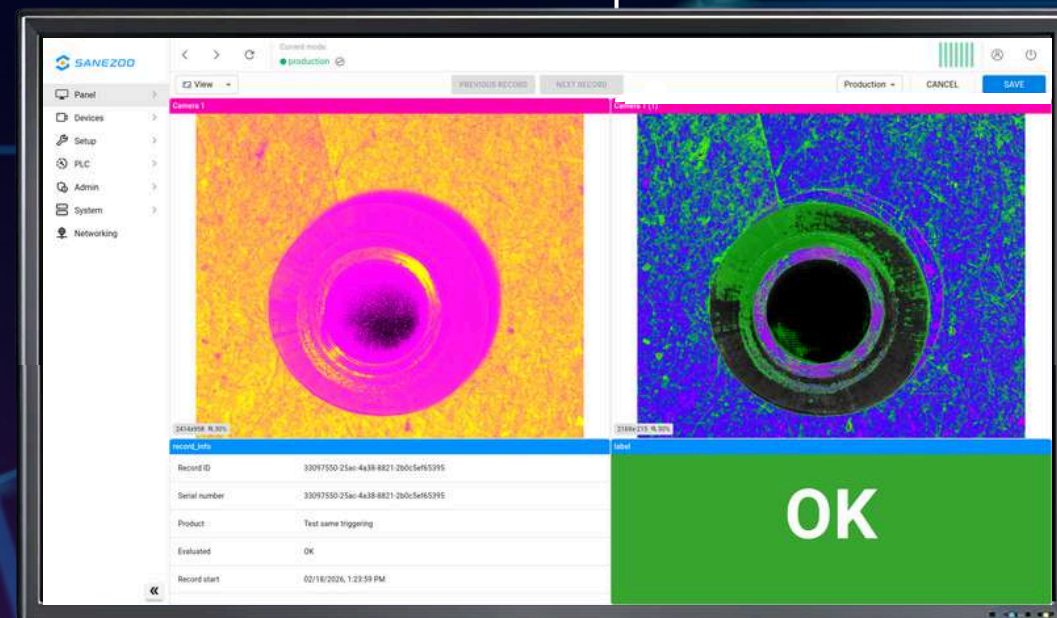
Anomaly detection
