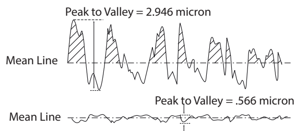
Fig. 10-15 Surface Roughness After Shot Peening and After C.A.S.E. TM Finishing
