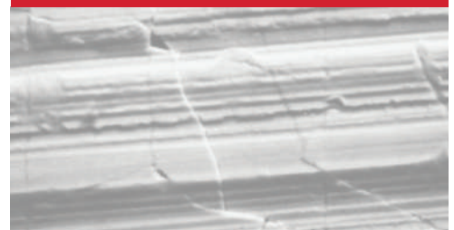
Fig. 3-3 Plating Micro-Cracks
