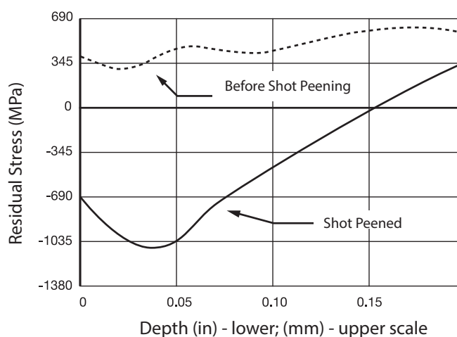
Fig. 5-3 Coil Spring ID Residual Stress With and Without Shot Peen
