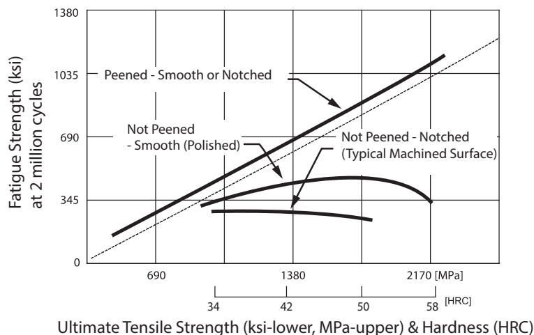
Fig. 2-1 Fatigue Strength vs. Ultimate Tensile Strength
