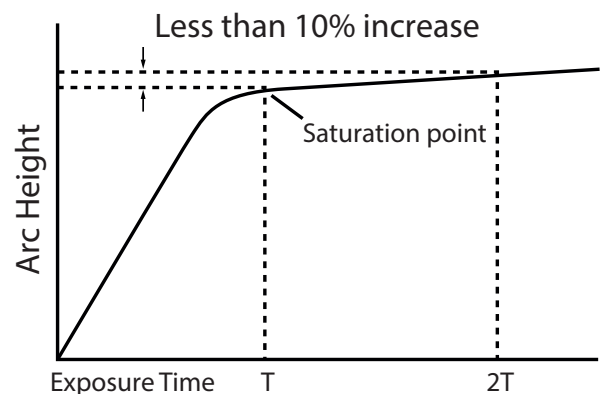
Fig. 11-7 Saturation Curve
