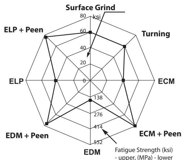
Fig. 3-5 High Cycle Fatigue Behavior of Inconel 718
