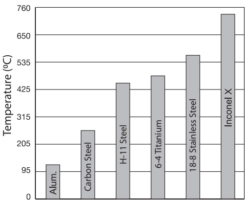
Fig. 9-2 Approximate Temperature at Which Compressive Stresses Begin to Dissipate
