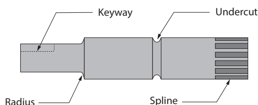
Fig. 5-4 Drive Shaft Schematic
