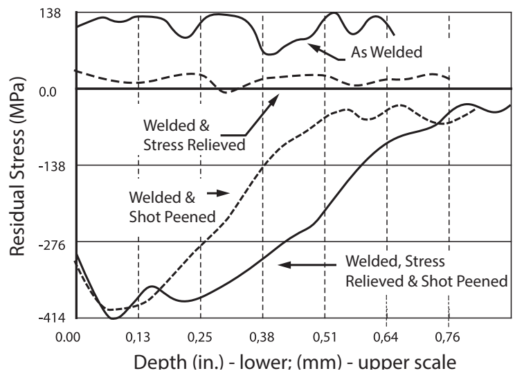
Fig. 3-1 Residual Stresses from Welding
