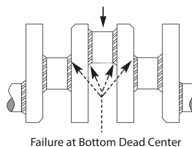
Fig. 4-6 Crankshaft Schematic
