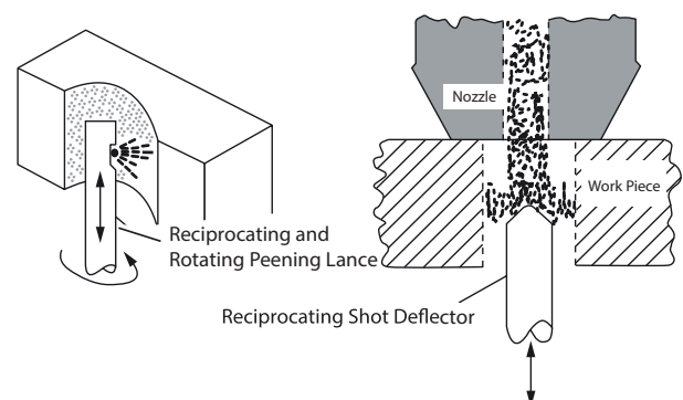
Fig. 10-9 Lance Peening and Internal Shot Deflector Peening
