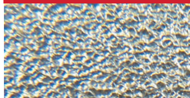
Fig. 11-8B Incomplete Shot Peening Coverage
