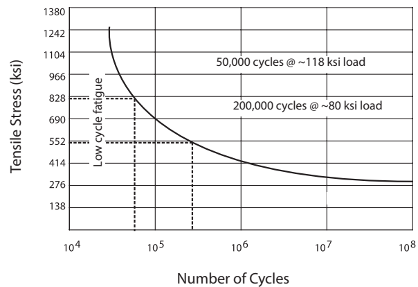
Fig. 1-4 Typical Stress vs Load Cycles
