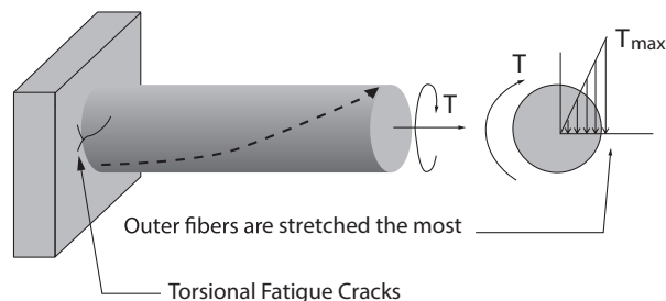
Fig. 5-1 Torsional Loading
