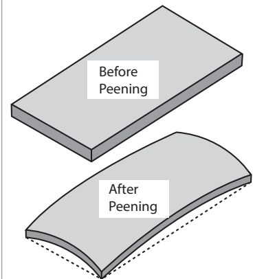
Fig. 10-1 Thin Cross Section Before and After Shot Peening
