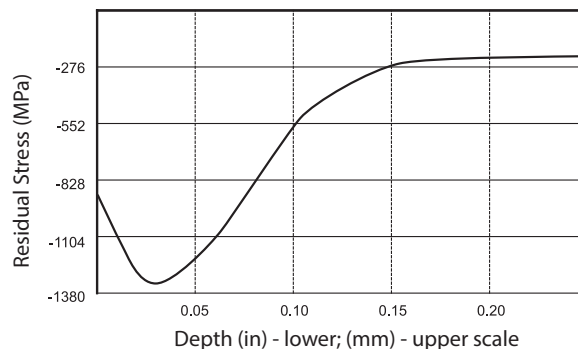
Fig. 4-4 Typical Carburized Gear Residual Stress Profile
