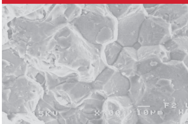
Fig. 8-3A SEM Photo of Intergranular Corrosion
