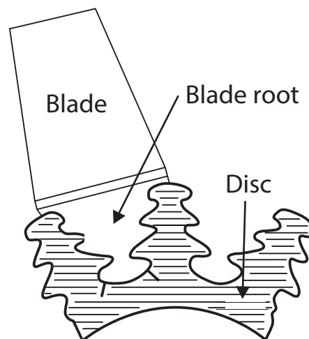
Fig. 7-2 Turbine Blade and Disc Assembly
