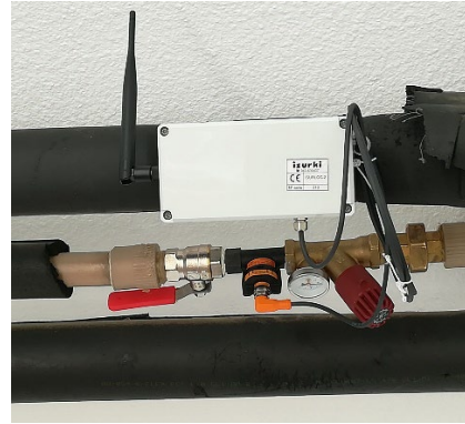
ISURLOG-LR deployed unit remotely monitoring flow and temperature on a hot water distribution network with LoRa comms.
