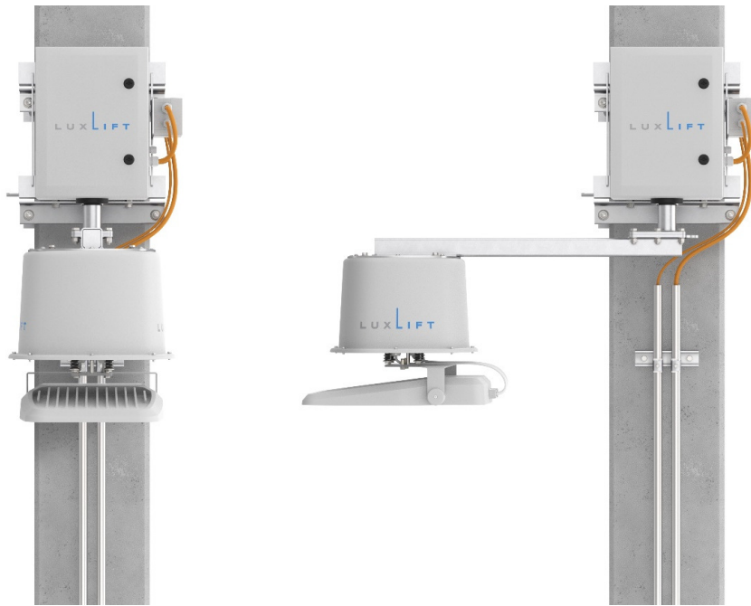
LuxLift Turn being rotated
