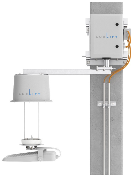
LuxLift Turn lowered for lamp maintenance
