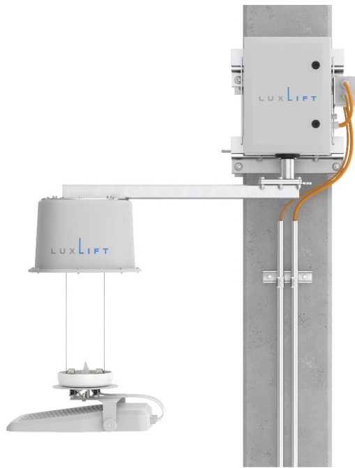
LuxLift Turn during lamp maintenance
