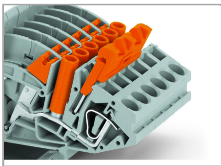
BJumper with safety lid in pre-locked position
