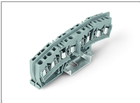
Separator for 3-conductor, double-potential terminal blocks (280-675)
