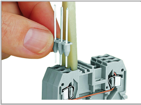
Inserting a pin module into 280 Series blocks.
