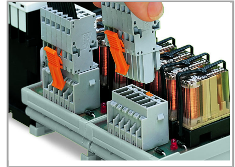
Pluggable PCB connection
