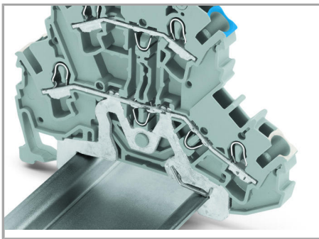
Both ground and shield conductor terminal blocks have a contact foot in the bottom level, automatically establishing direct contact to the carrier rail or busbar.
