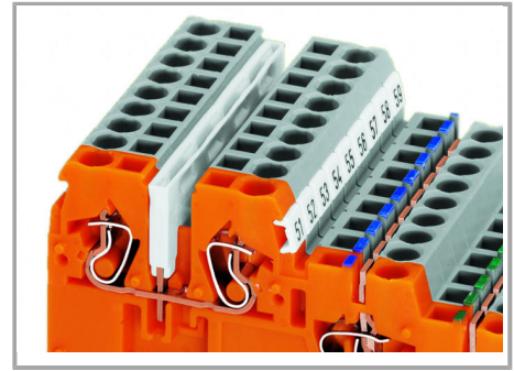
Commoning signal level voltage via insulated push-in type jumper bars (870 Series) – 2- to 9-way, depending on application.
