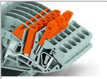
B Jumper with safety lid in pre-locked position
