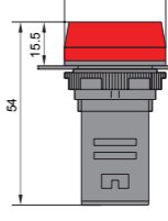
Ex9PB
