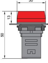
Ex9IL 1
