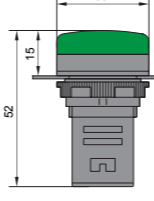
Ex9IL 2
