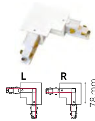
L CONNECTOR
