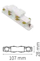
ELECTRIFIED CONNECTOR
