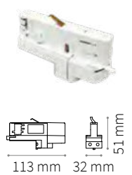
TRACK CONNECTOR
