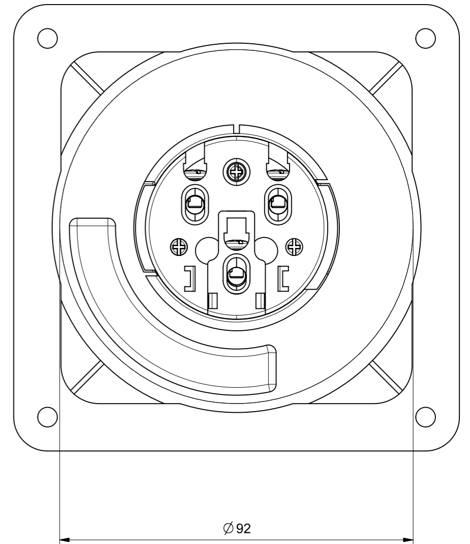
FORATURA PANNELLO // PANEL DRILLING HOLE
